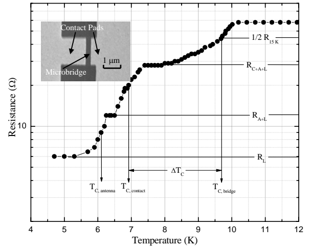
Fig. 3. Resistance versus temperature curve of the measured HEB device, R_{C+A+L} is the resistance above T_{c,contact} with T_{c,contact} the critical temperature of the stack layer containing the contact pads and antenna structure on top of the NbTiN film, R_{A+L} the resistance of the antenna and leads, T_{c,bridge} the critical temperature of the NbTiN microbridge, R_L the leads resistance, and \Delta T_C the transition width. Inset: zoomed SEM micrograph of the NbTiN microbridge between the contact pads.
