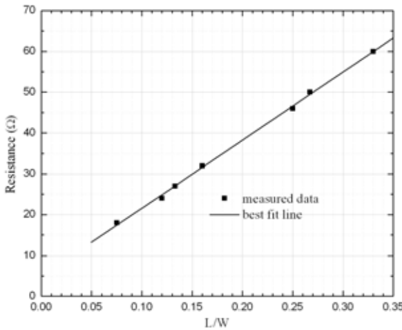
Fig. 2. Measured normal state resistance at 15 K ( R_{15K} ) as a function of the ratio of the microbridge length to the width ( L/W ). The square resistance ( R_{,15K} ) at 15 K is evaluated to be about 170 \Omega from the slope of the best fit line.
